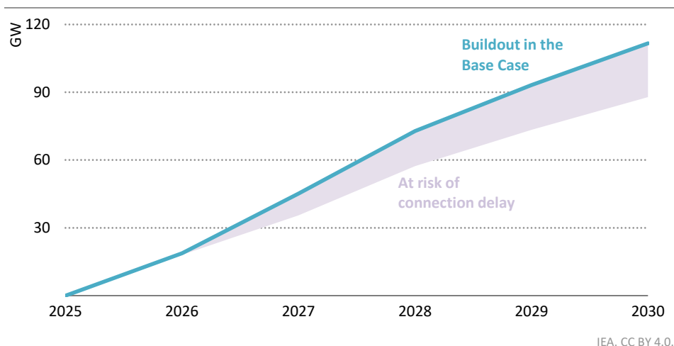
Figure 2.27 ▶ Global data centre capacity in the Base Case and capacity at risk of connection delay due to grid constraints, 2025-2030
