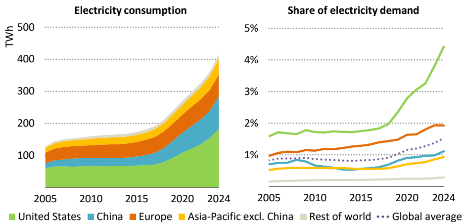
Figure 2.6 ▶ Electricity consumption of data centres by region, 2005-2024
