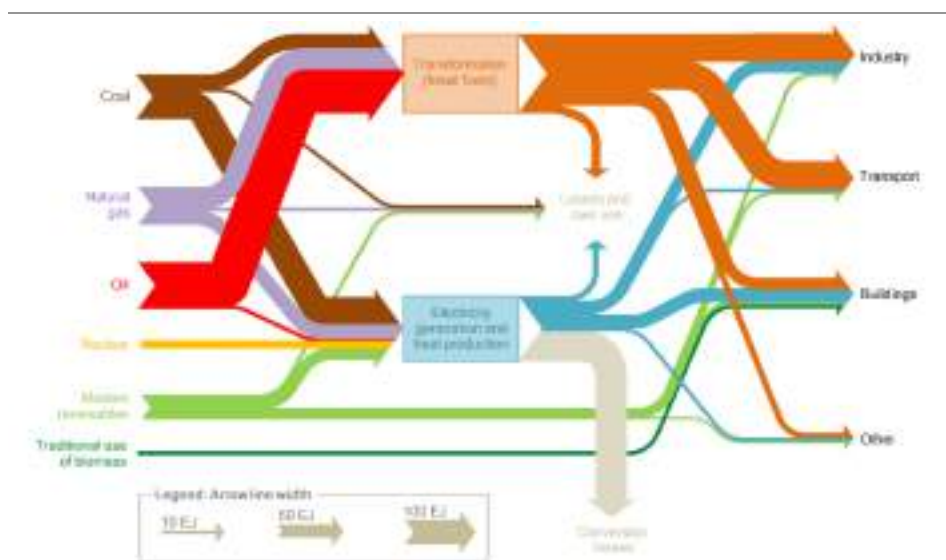
Figure 3.1 ▶ Energy supply, transformation and end-use, 2024
