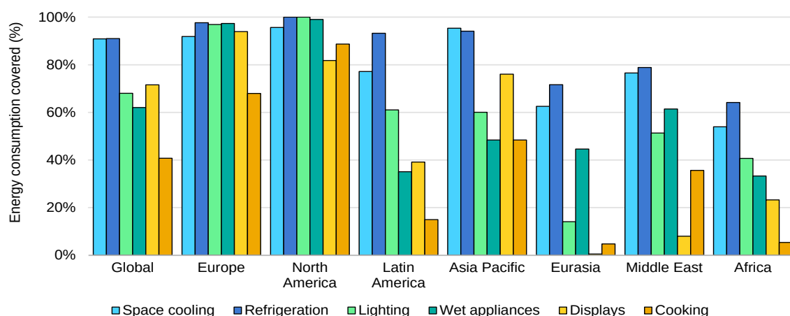
Energy use coverage of minimum energy performance standards for appliances by region, 2025
