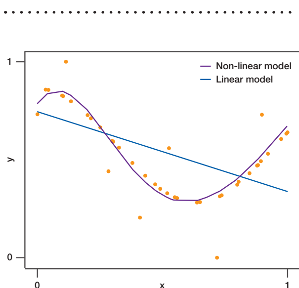
Figure 4-2 | Regression
