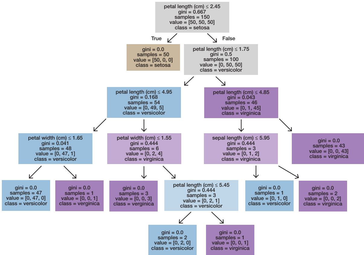
Figure 4-5 | Decision tree
