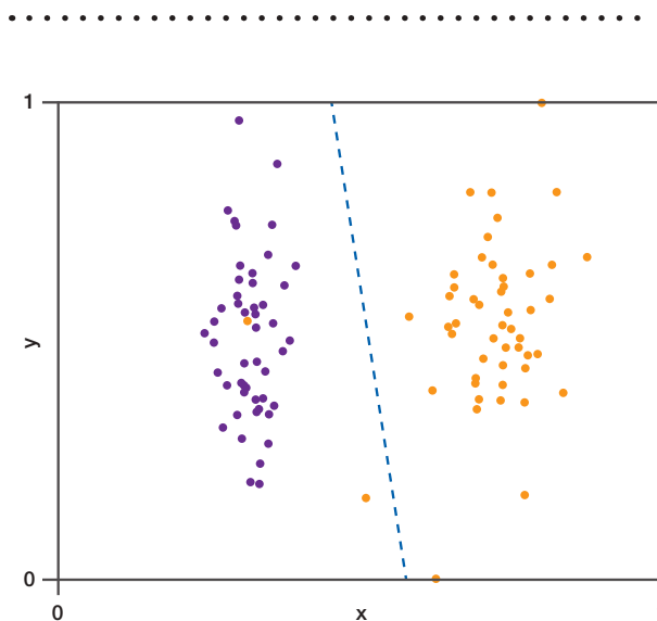
Figure 4-1 | Classification
