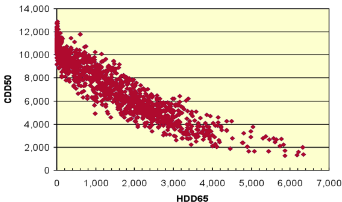
Figure 1. Distribution of areas by heating and cooling degree-days (HDD65 y CDD50) for 1,400 locations in Mexico
